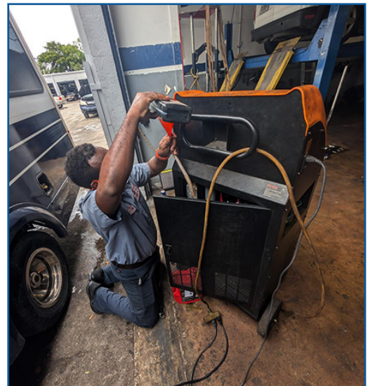
FTTP trainer Eddie Patane made a trip to F A Fleet in Margate recently and conducted an HVAC training session and also assisted the shop with an AC repair while there. F A Fleet staff involved during the day were Floyd Thompson, owner, Jabaree Foster and Steve Smith.
